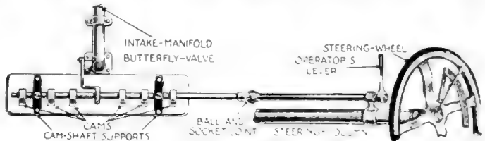
At the rear end of a camshaft a ball-and-socket joint connects with a shaft that leads to the operating lever
